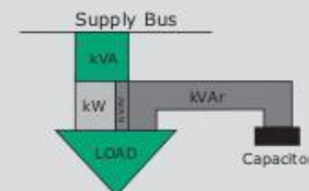
Figure 3 : Network with capacitor
